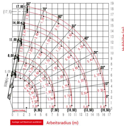
Lastdiagramm (t)
