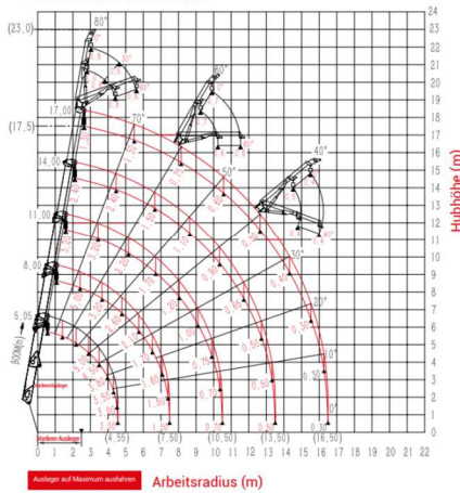
Lastdiagramm (t)
